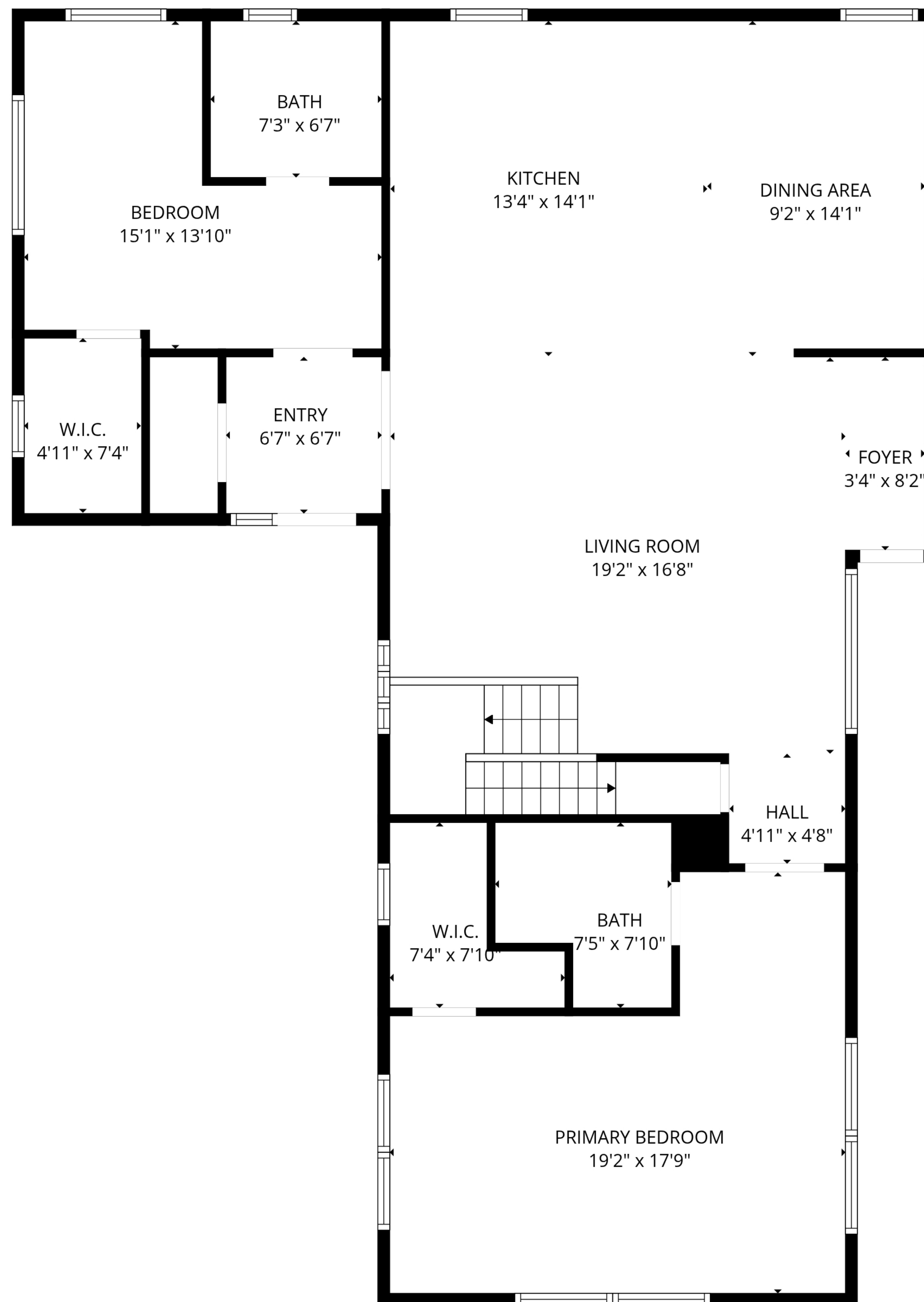
1st floor
