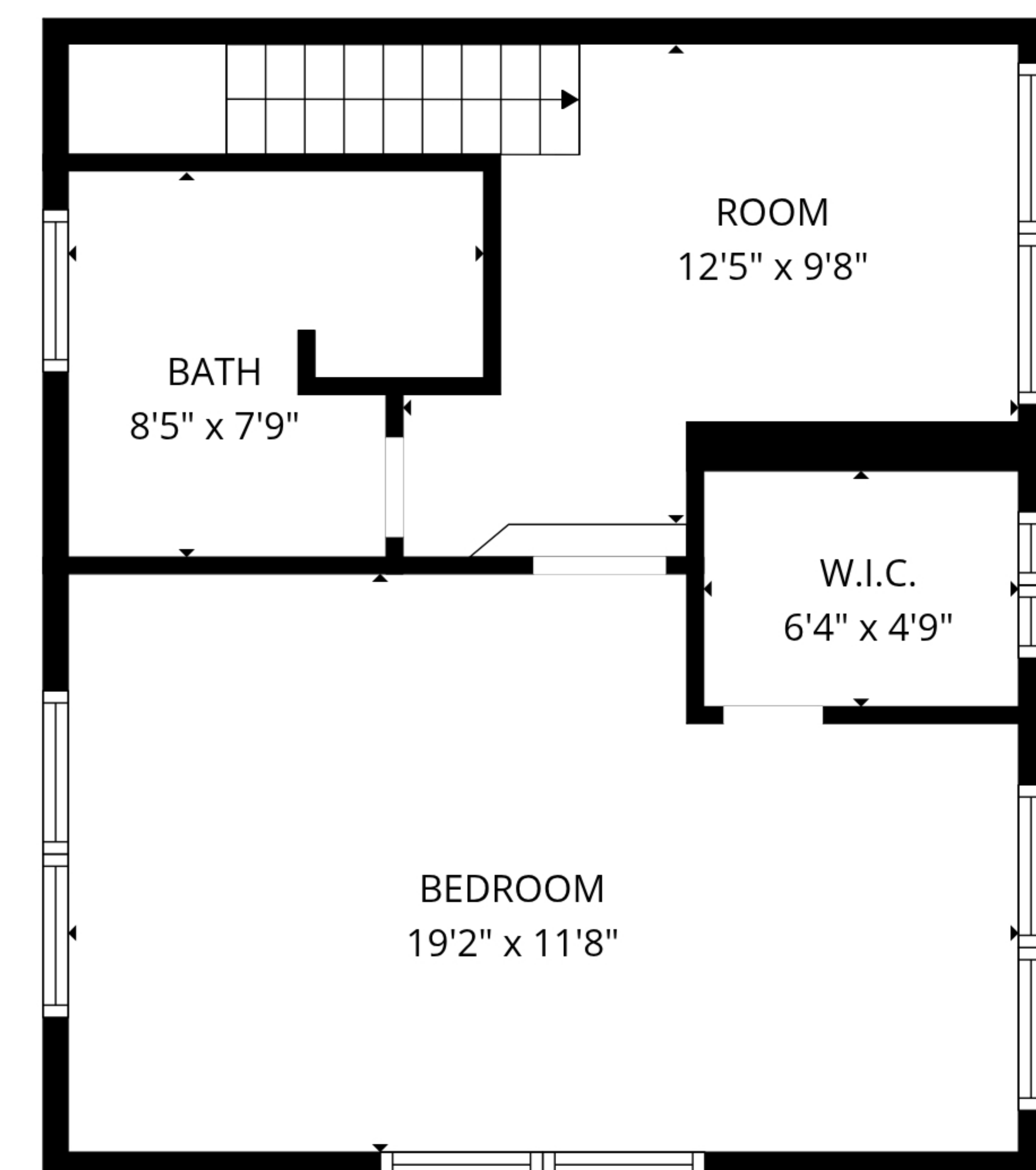
2nd floor
